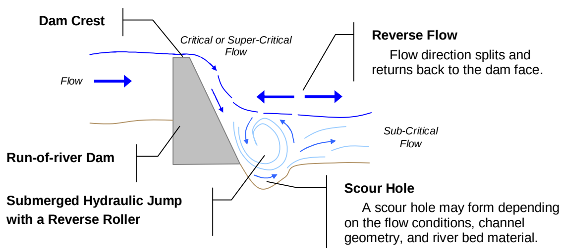
Figure 1.7-2 - Submerged Hydraulic Jump
