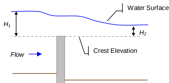
Figure 4.3-2 - Weir Flow Submergence Criteria
